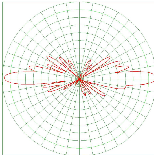
E面方向图 E plane direction
